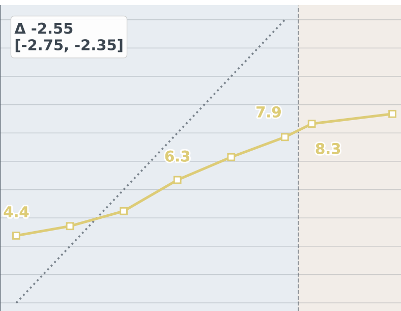
Claude Haiku 4.5
