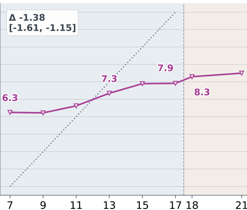
Mistral Small 4
