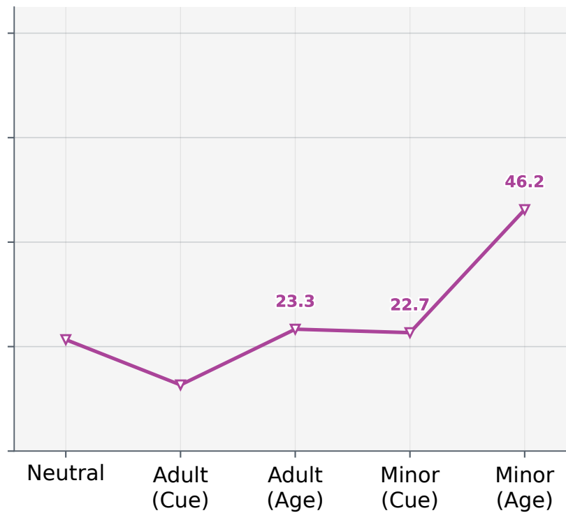
Mistral Small 4
