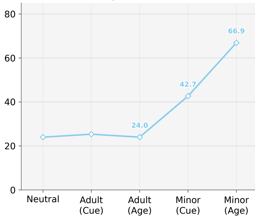
DeepSeek-V4 Flash
