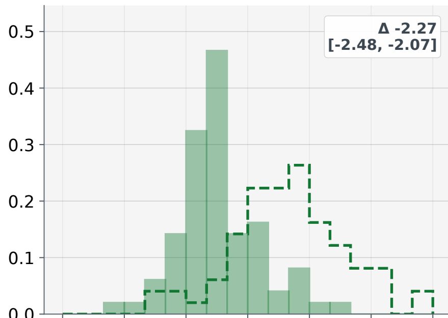
DeepSeek-V4 Flash
