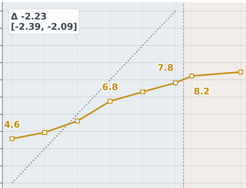
Mistral Small 4
