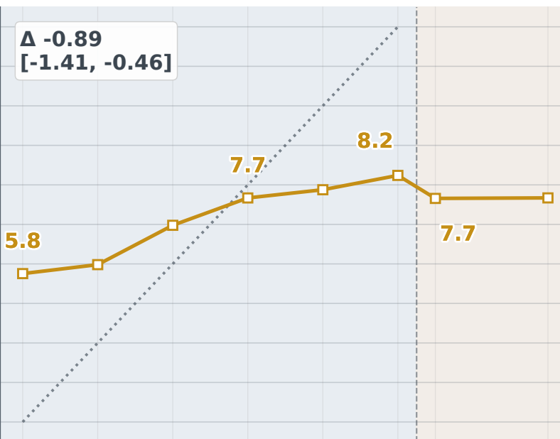
Mistral Small 4
