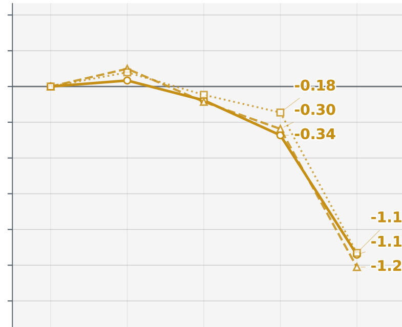
Mistral Small 4
