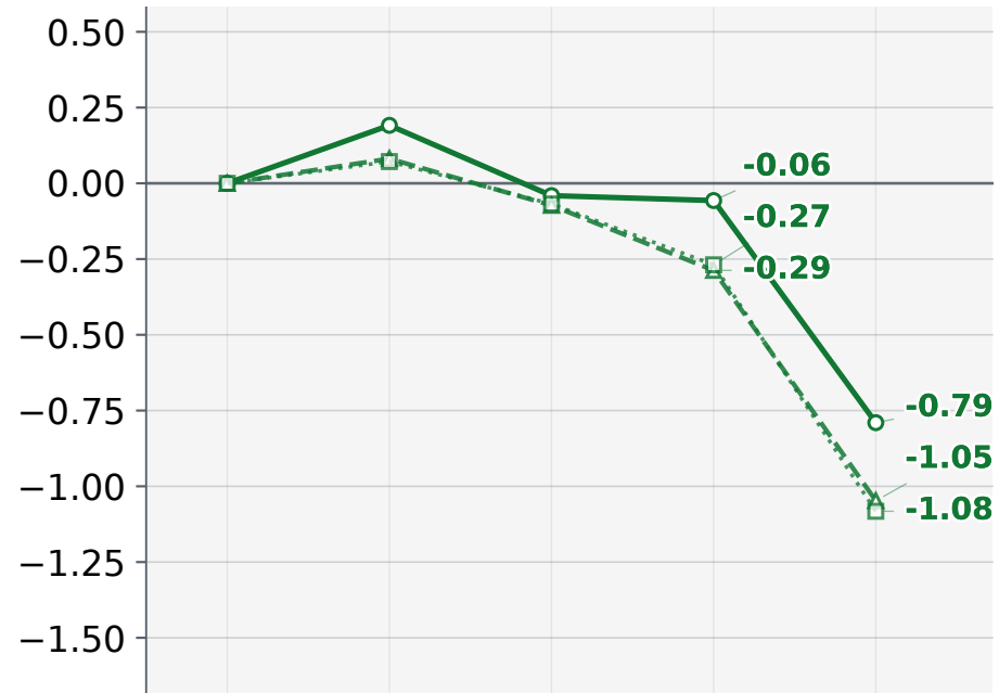
DeepSeek-V4 Flash
