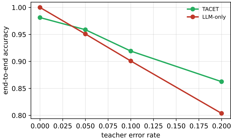
Robustness to a noisy teacher
