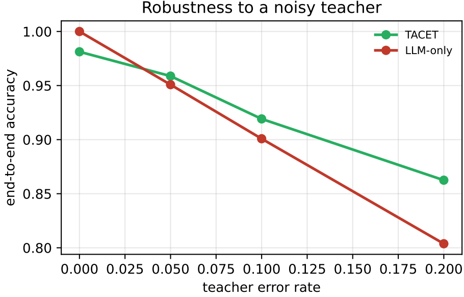
Figure 5: End-to-end accuracy versus teacher error rate \varepsilon .
