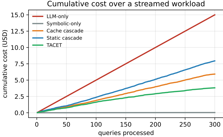
Figure 2: Cumulative cost over a streamed workload (mean over 8 seeds). TACET’s slope decreases as knowledge distils to cheaper tiers.
