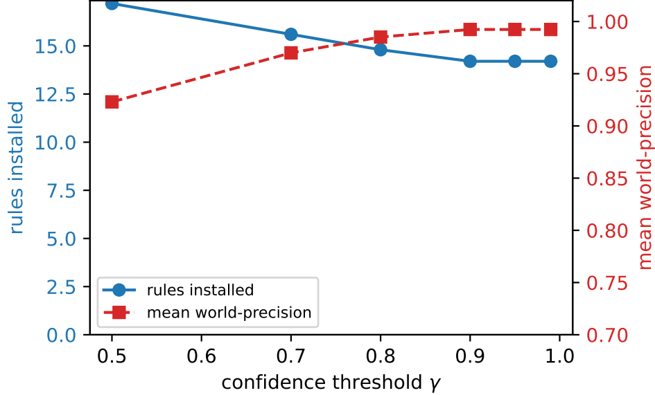
Figure 1: Confidence-threshold ( \gamma ) sensitivity on the synthetic benchmark (oracle teacher, mean over five seeds). As \gamma rises, fewer rules install (left axis) but the mean world-precision of the survivors rises (right axis) — the homophily relations are the last to be filtered out.
