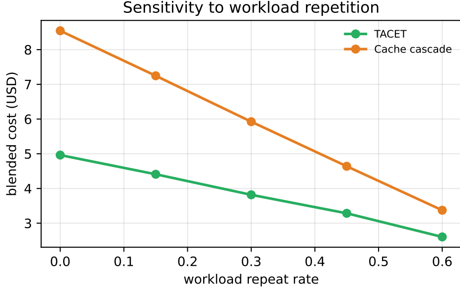
Figure 4: Blended cost versus workload repeat rate. The cache rises steeply toward the LLM-only regime as repetition vanishes; TACET degrades gently because synthesised rules and the KGE generalise to unseen entities.
