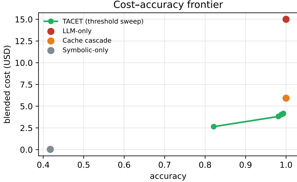
Figure 3: Cost-accuracy frontier. The curve is TACET swept over the Tier-2 confidence threshold \theta ; markers are baseline systems.
