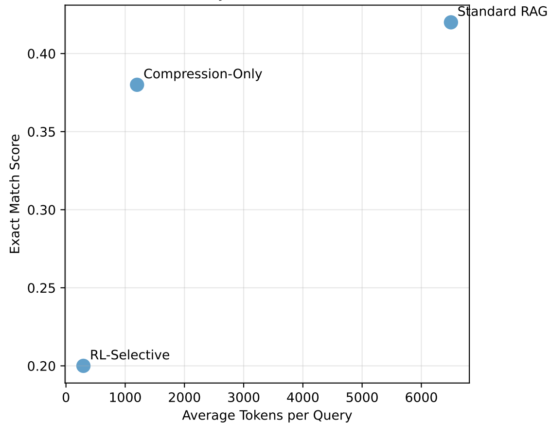
Quality vs Cost Trade-off
