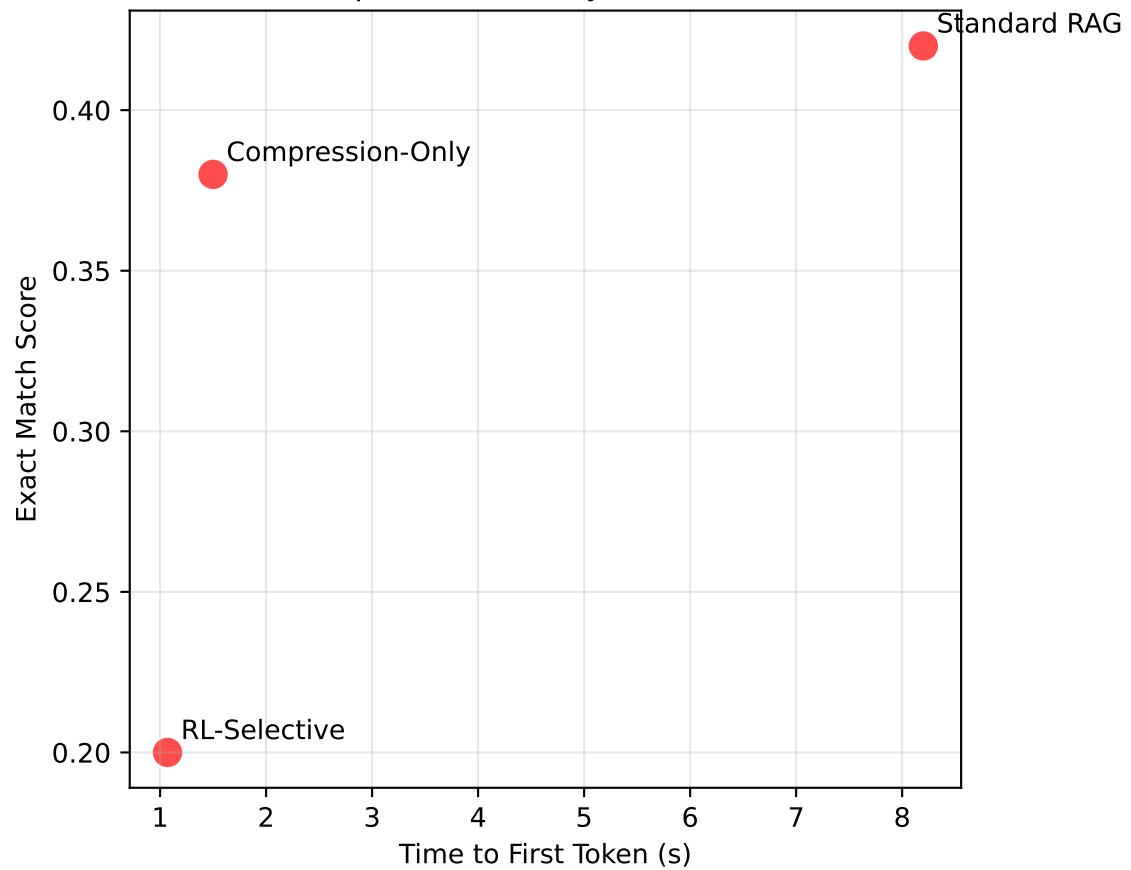
Speed vs Quality Trade-off
