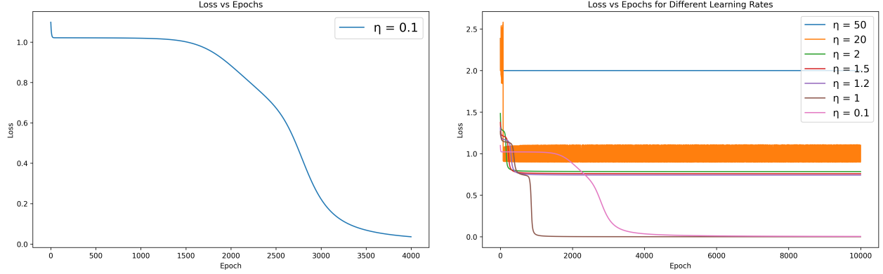
(a) Loss vs Epoch Curve for \eta = 0.1 , Trained for 4000 epochs (b) Loss vs Epoch curve for Varying \eta , Trained for 10000 epochs
