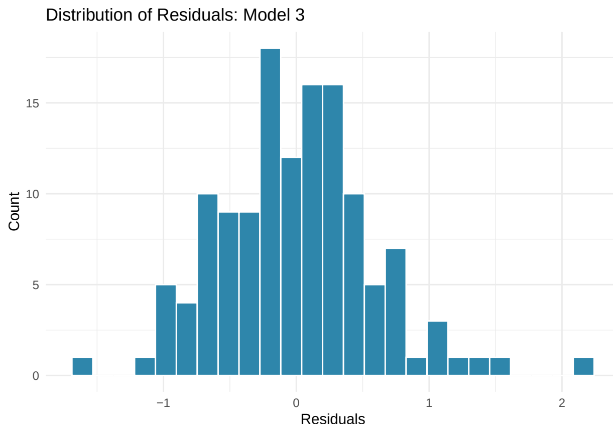
Figure 4 shows the distribution of residuals from Model 3. The approximately bell-shaped, symmetric distribution centered near zero suggests the normality assumption is reasonably met, supporting the validity of the model's inference.
