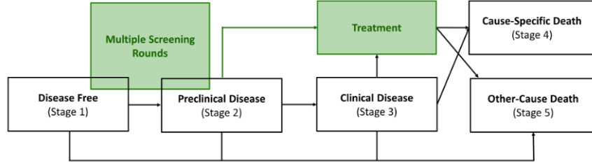
Figure 2: Screening model diagram taken from Lin, O’Mahony, and Rosmalen (2023). The white health states represent the natural history of disease. The two interventions, screening and treatment, are labelled in green. The screening intervention can only be implemented before the individual enters clinical health state (stage 3), and treatment can be received when patients are diagnosed from screening (stage 2) or clinically presented (stage 3).
