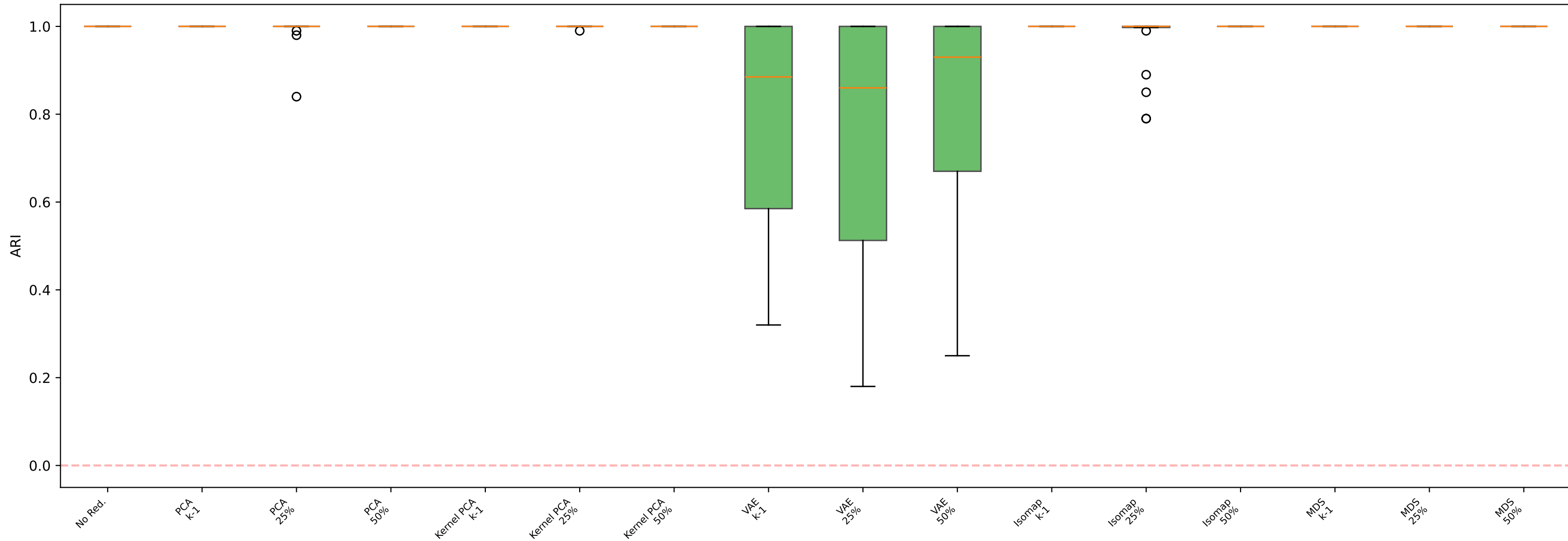
AHC — Repliclust
