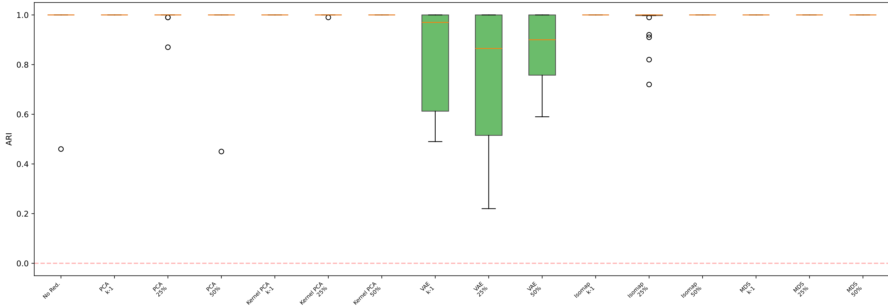
GMM — Repliclust
