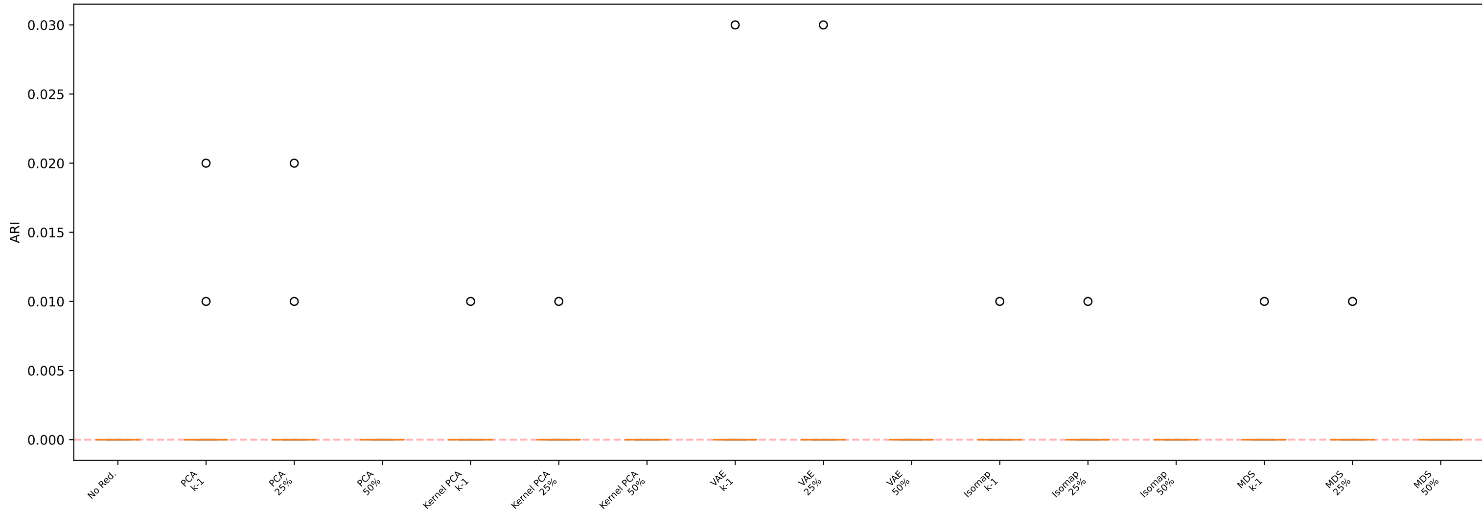
OPTICS — Circles
