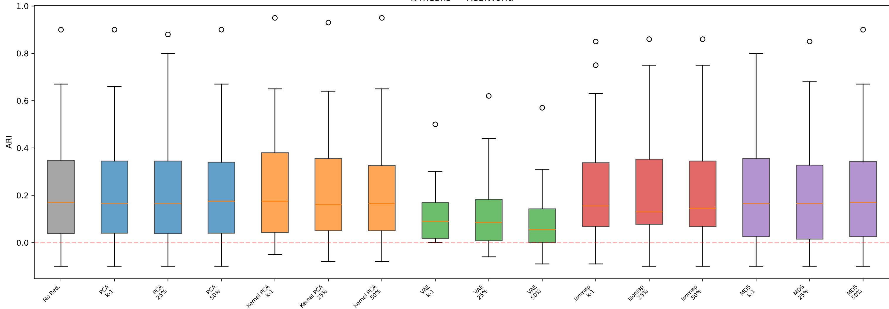
k-means — RealWorld
