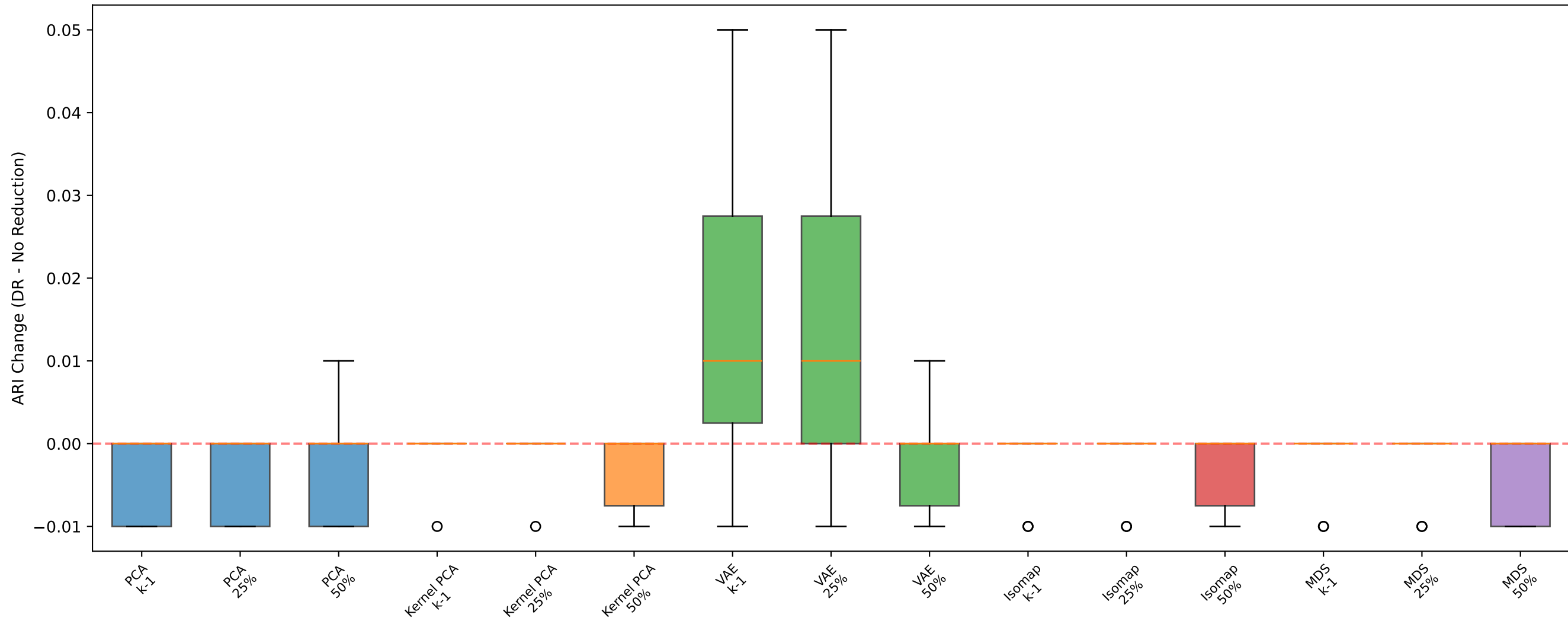
AHC - Circles: ARI Change by DR Method
