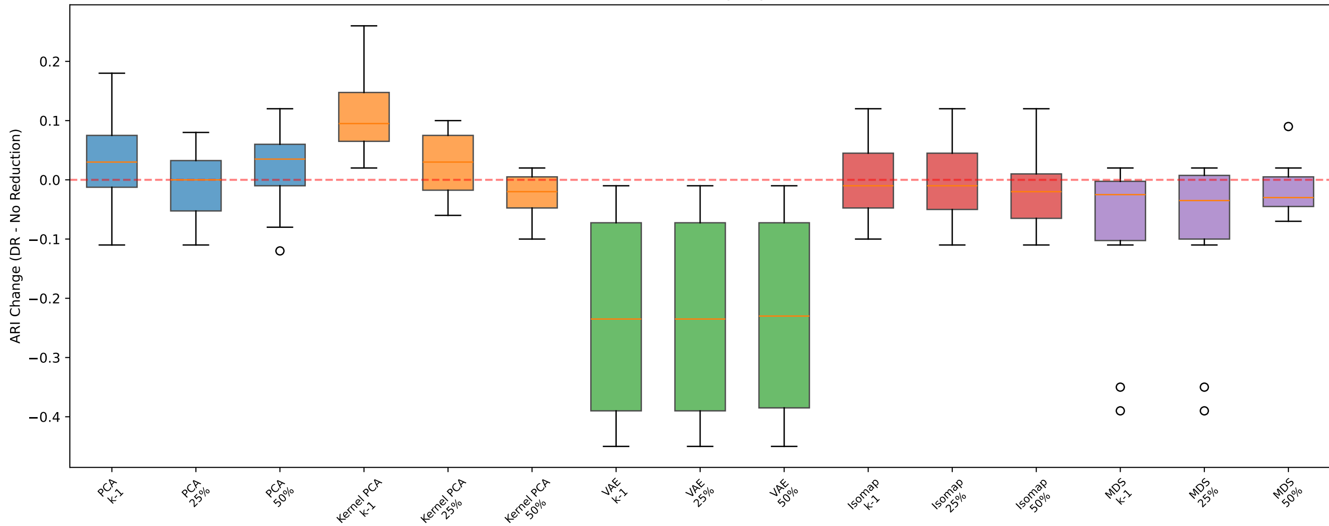
AHC - Moons: ARI Change by DR Method
