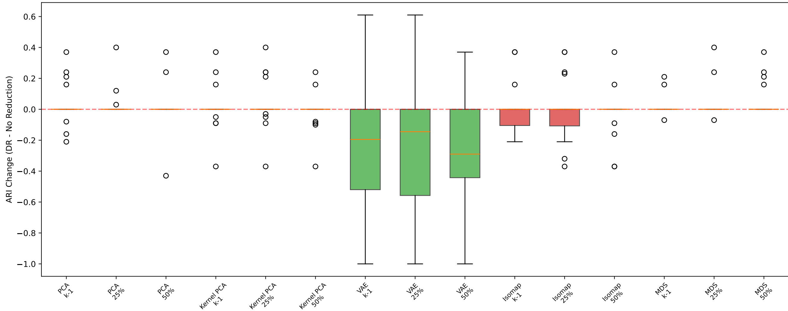
OPTICS - RSG: ARI Change by DR Method
