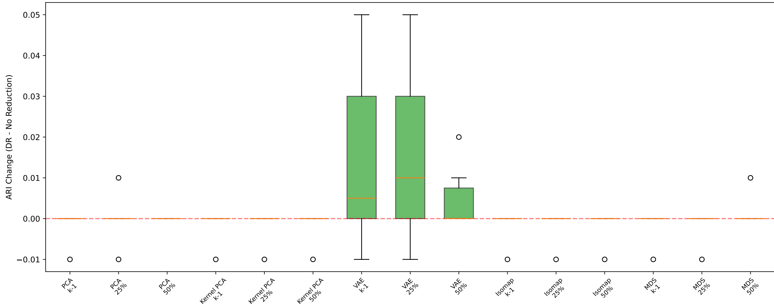
k-means - Circles: ARI Change by DR Method
