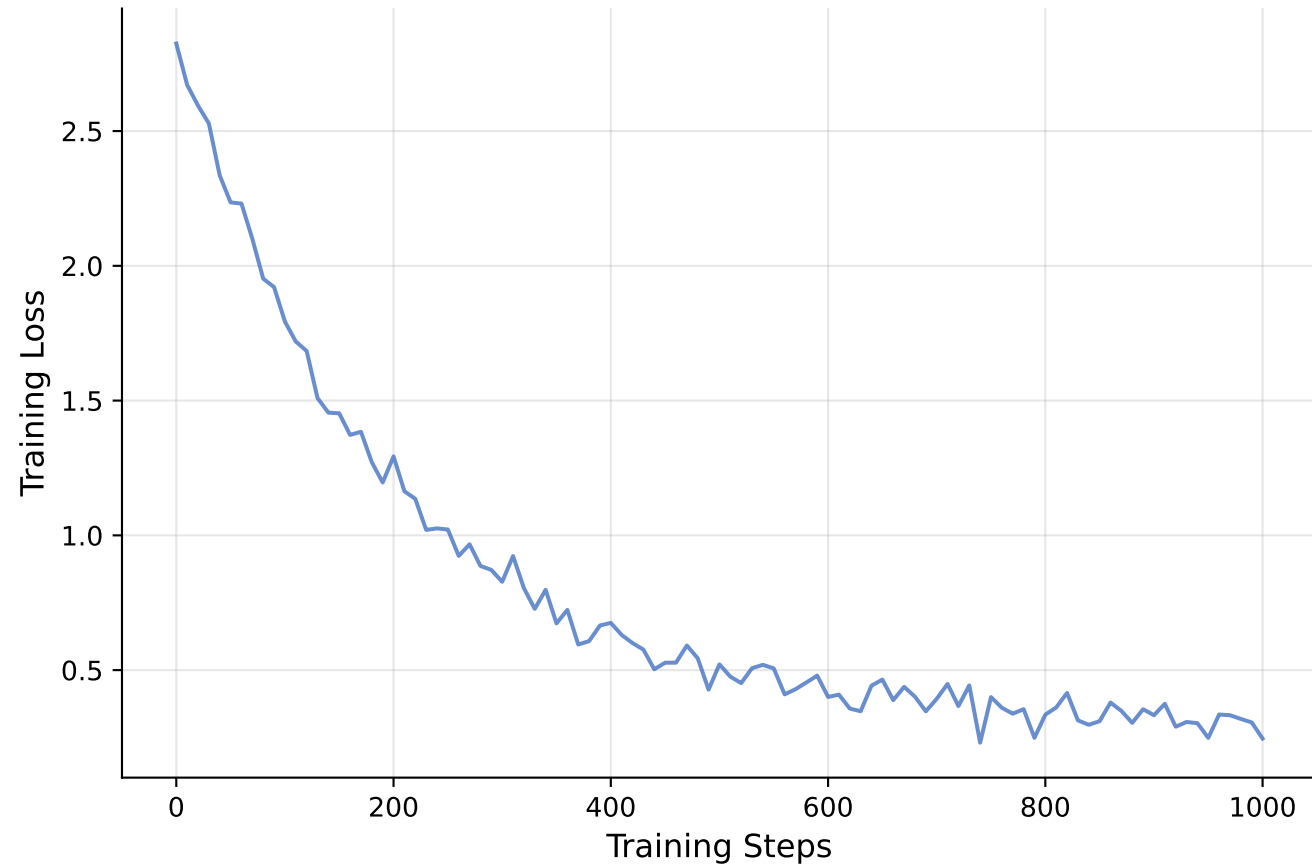
SFT Training Loss (1 epoch, batch=128)
