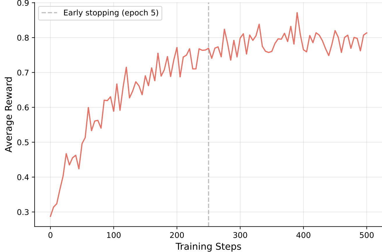
GRPO Training Reward (5 epochs, early stopped)
