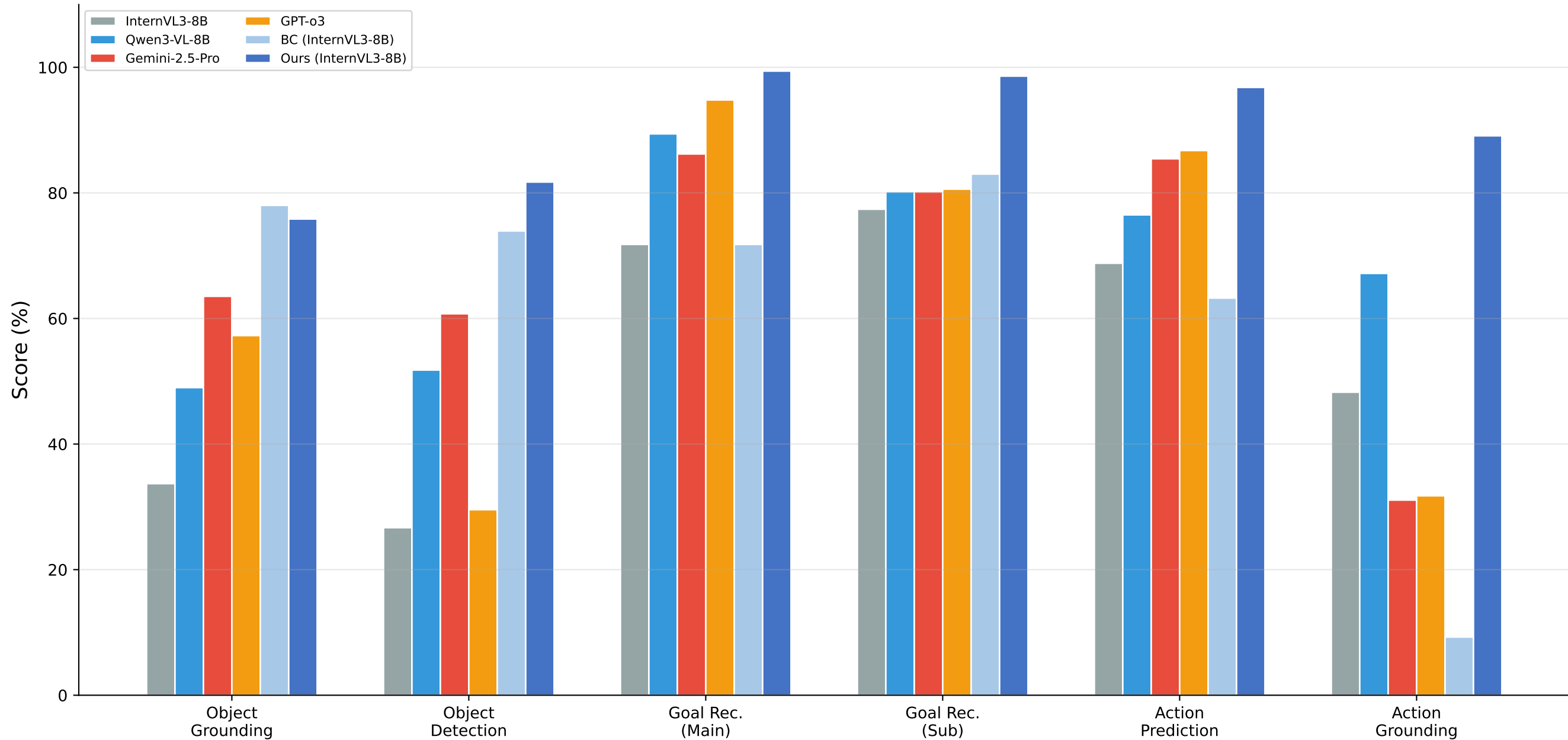
Skill Evaluation Comparison on ALFRED
