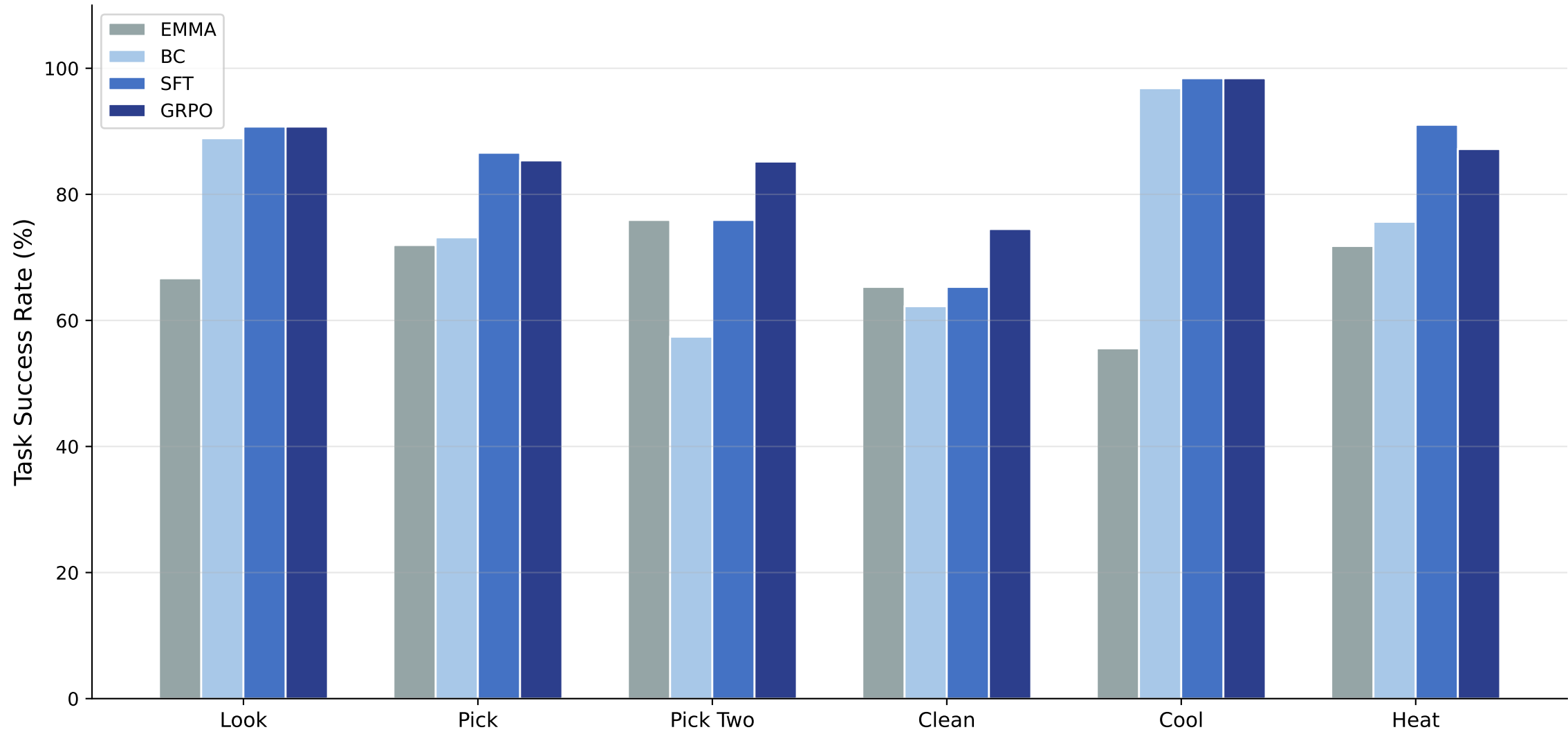
Per-Task-Type Success Rate Comparison
