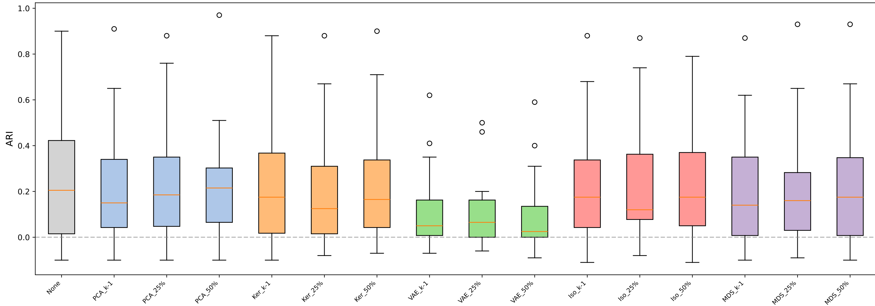
GMM - Real-World
