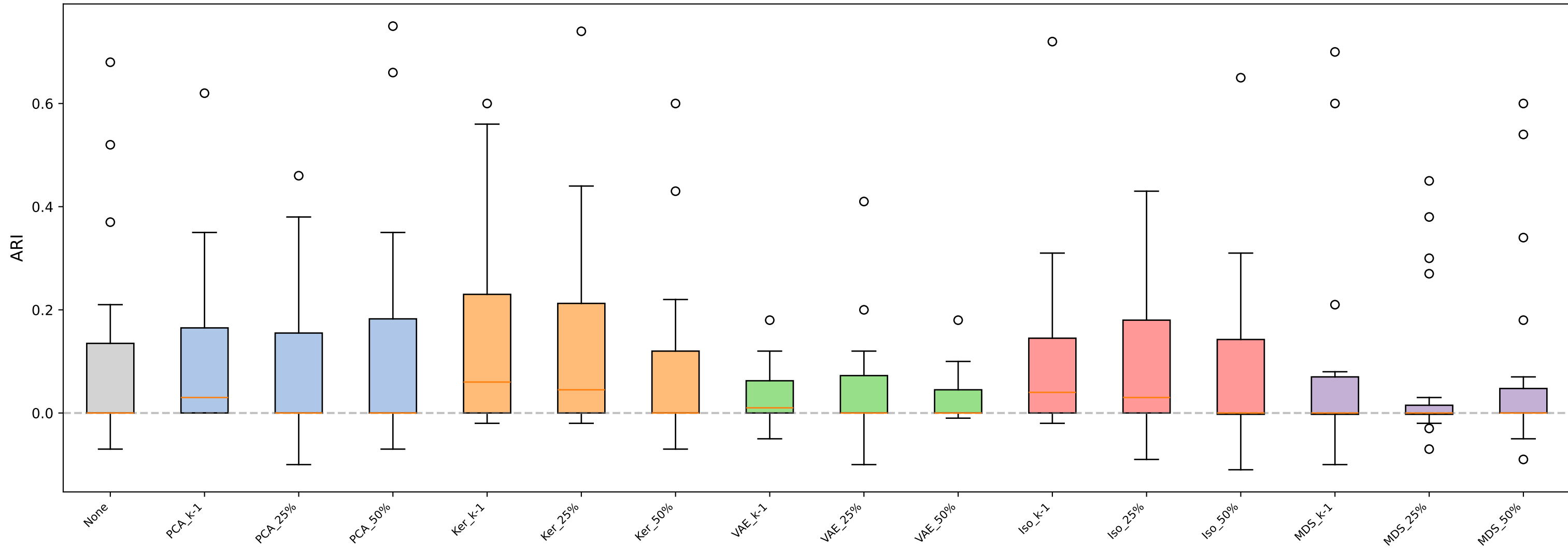
OPTICS - Real-World
