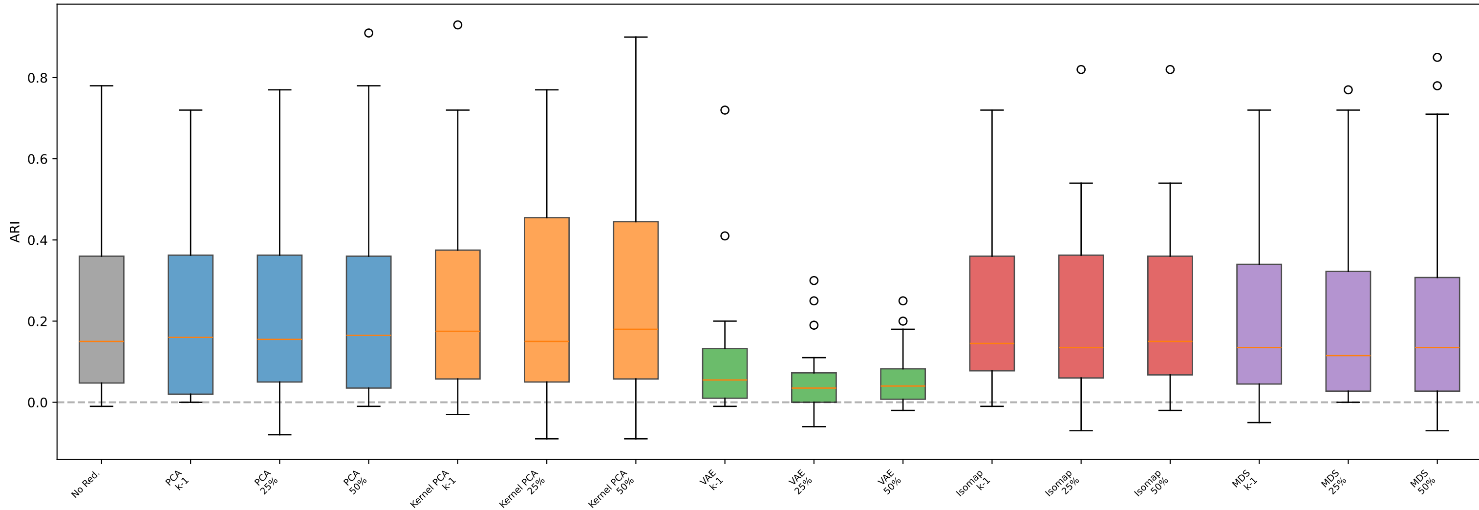
AHC — RealWorld
