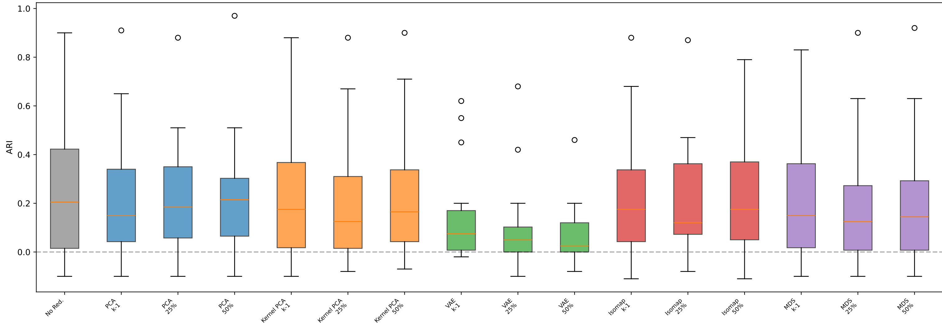
GMM — RealWorld
