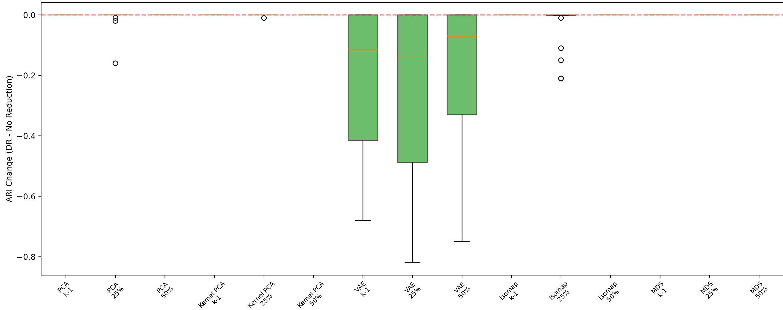
AHC - Repliclust: ARI Change by DR Method
