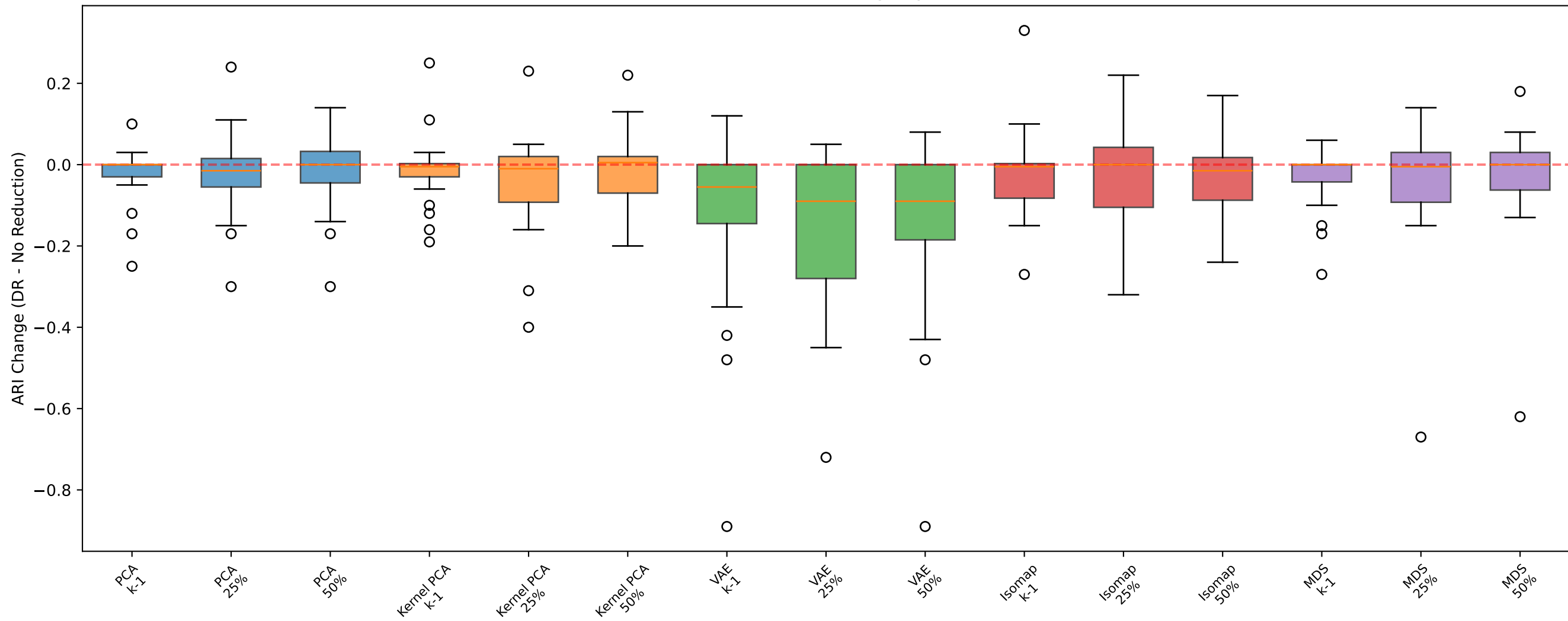
GMM - RealWorld: ARI Change by DR Method
