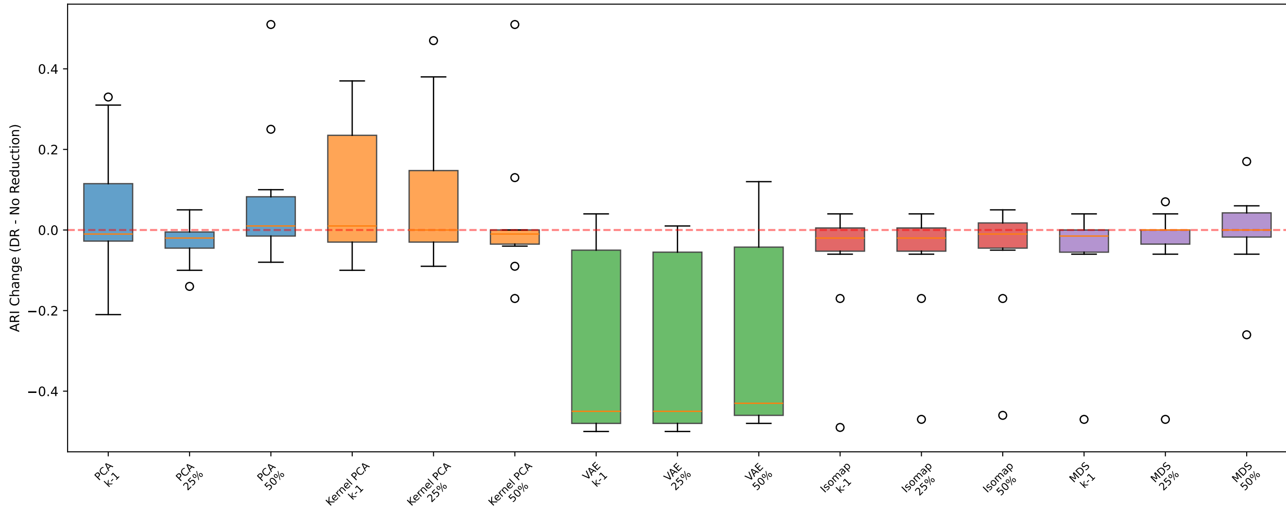
GMM - Moons: ARI Change by DR Method
