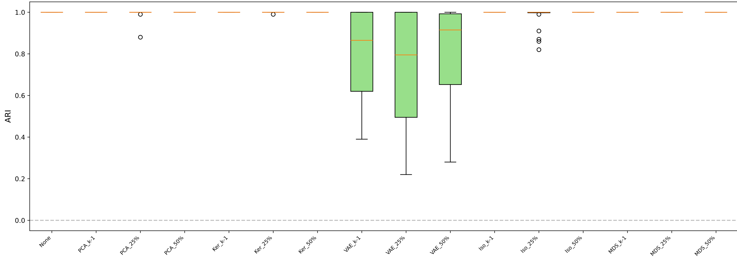
k-means - Synthetic (Repliclust)
