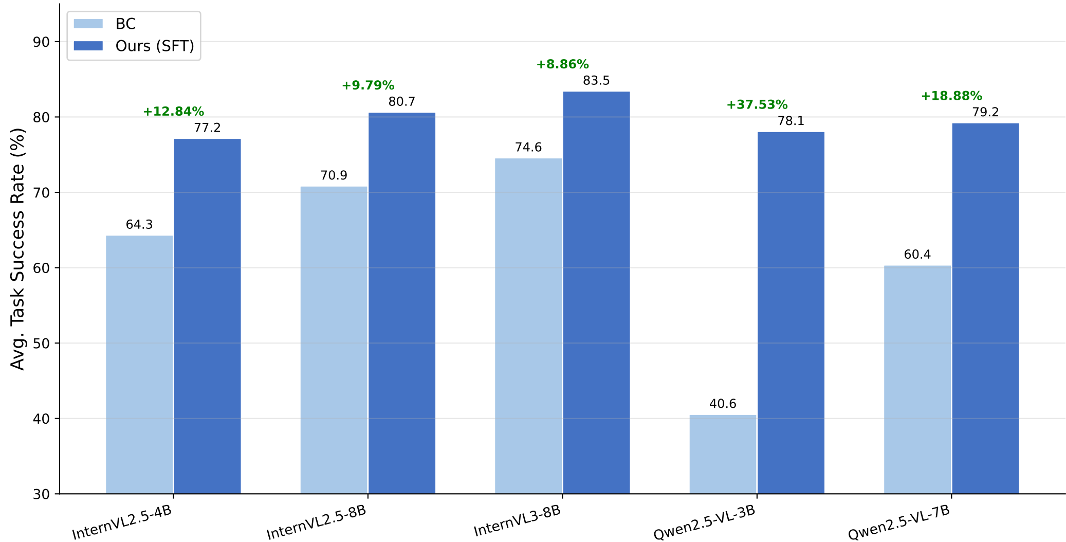
Comparison of VLM Backbones on Task Evaluation (SFT Stage)
