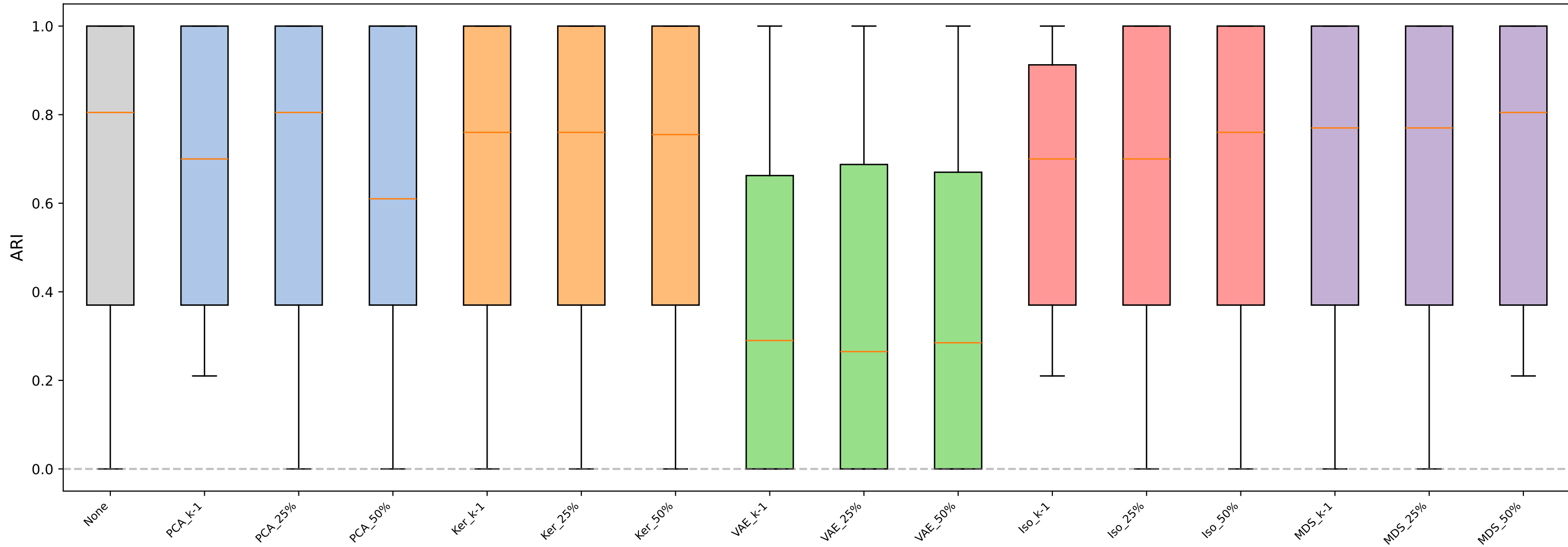
OPTICS - Synthetic (RSG)
