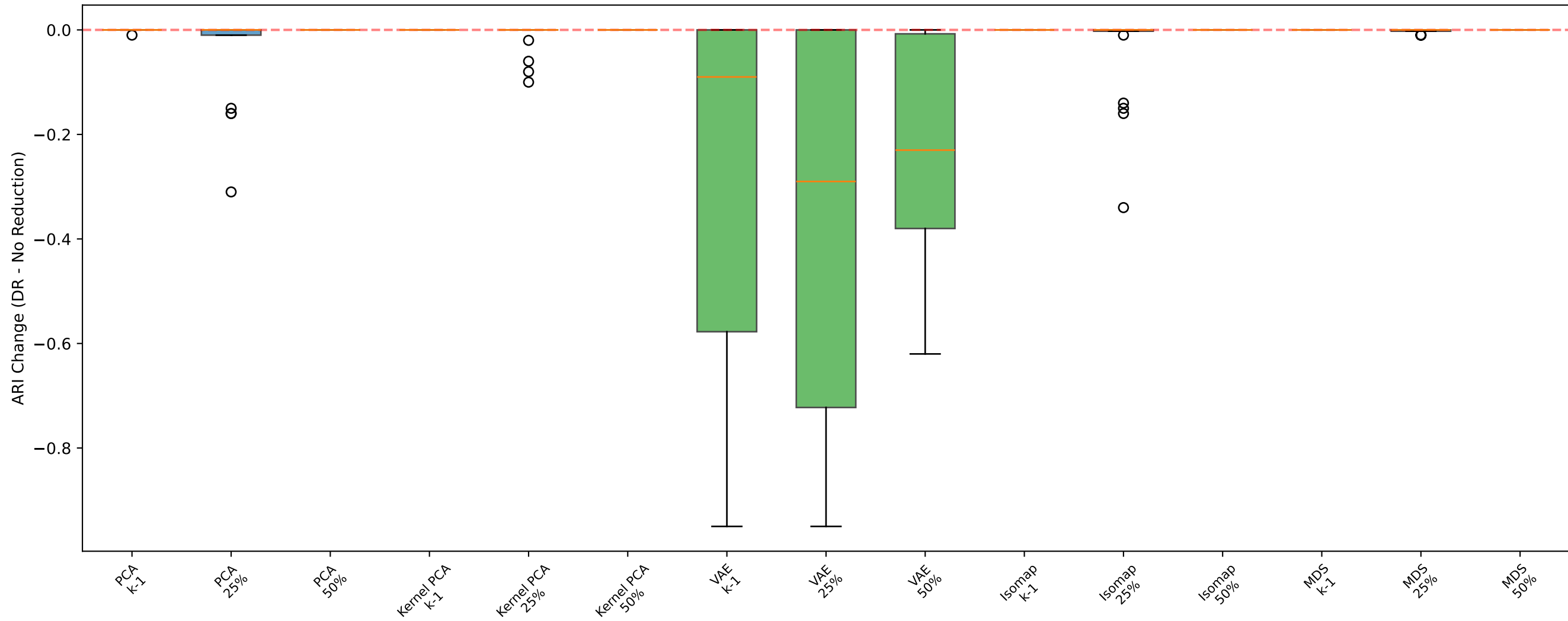
AHC - RSG: ARI Change by DR Method
