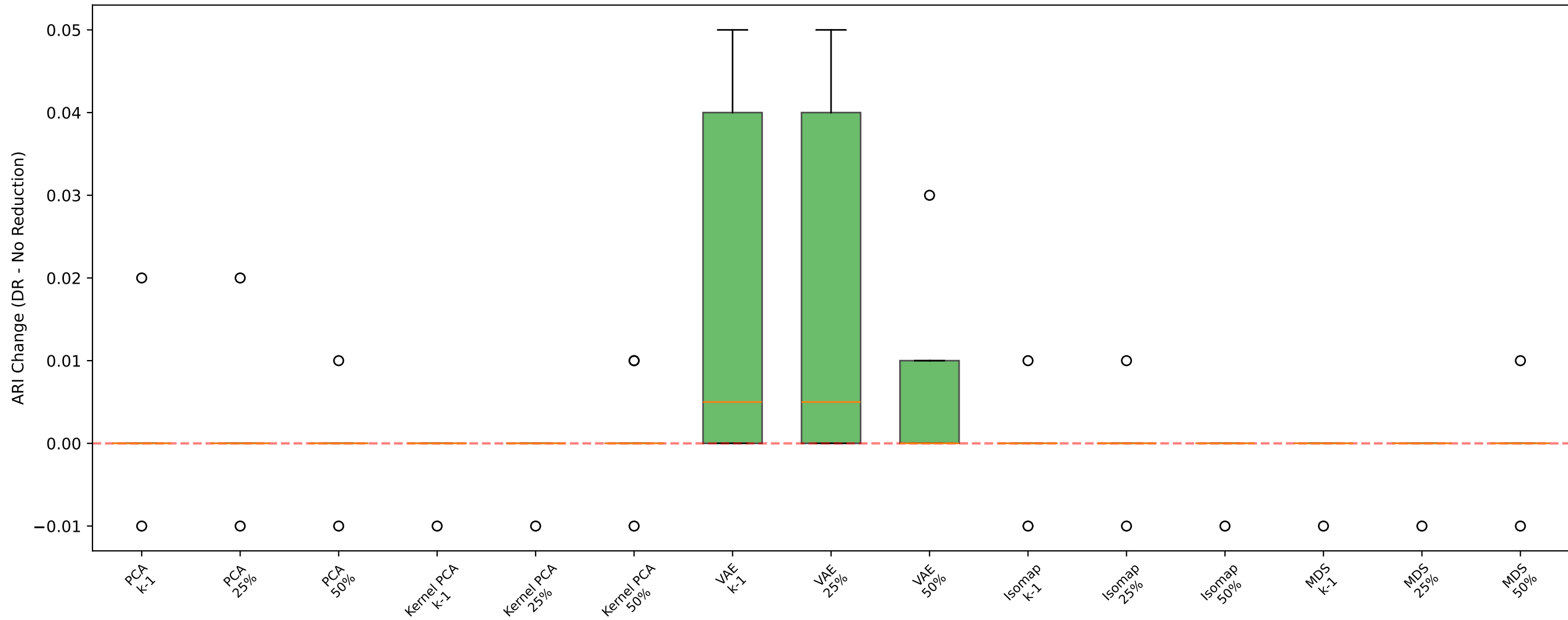
GMM - Circles: ARI Change by DR Method
