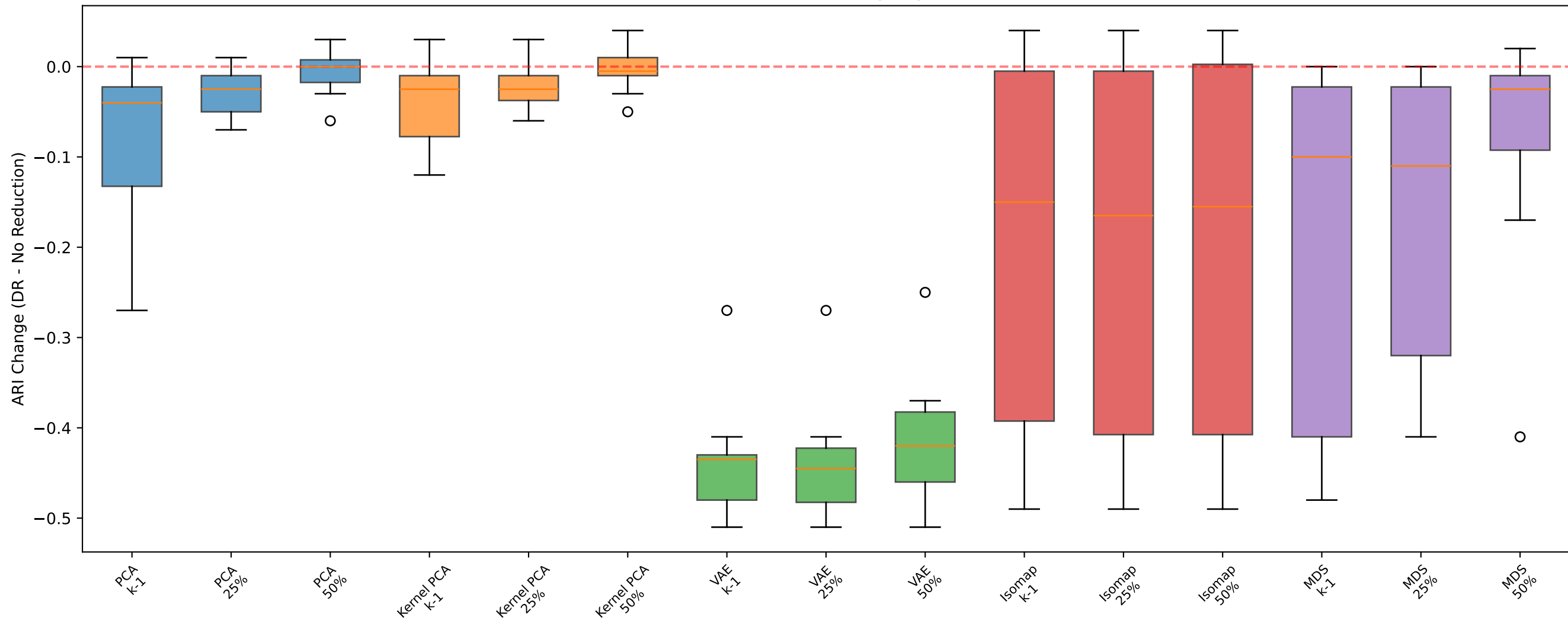
k-means - Moons: ARI Change by DR Method
