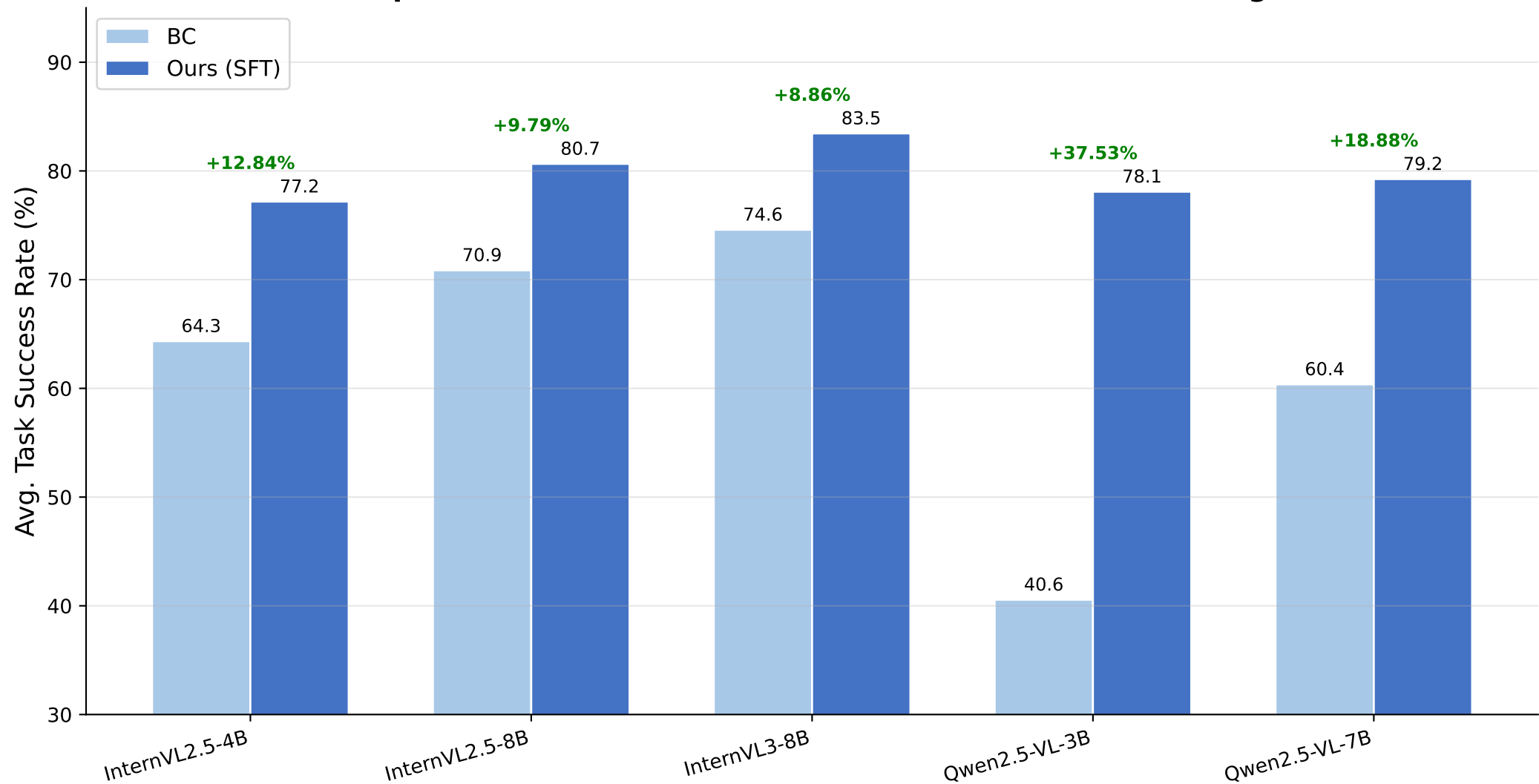
Comparison of VLM Backbones on Task Evaluation (SFT Stage)
