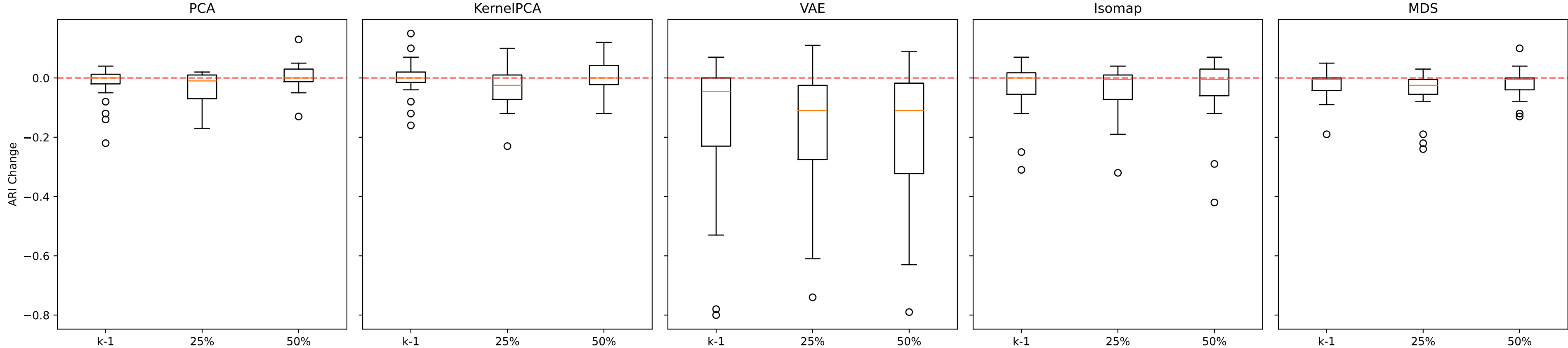
AHC - ARI Change with DR (Real-World)
