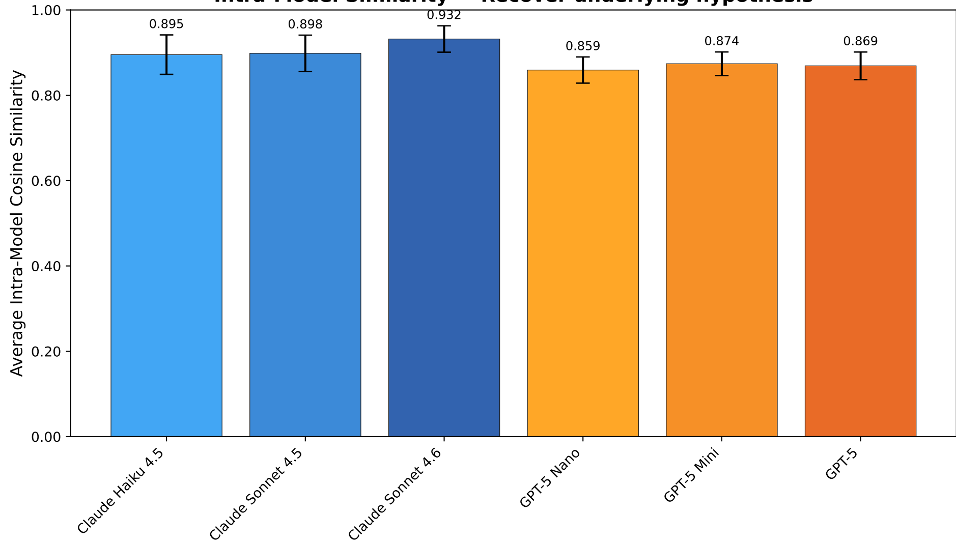
Intra-Model Similarity — Recover underlying hypothesis
