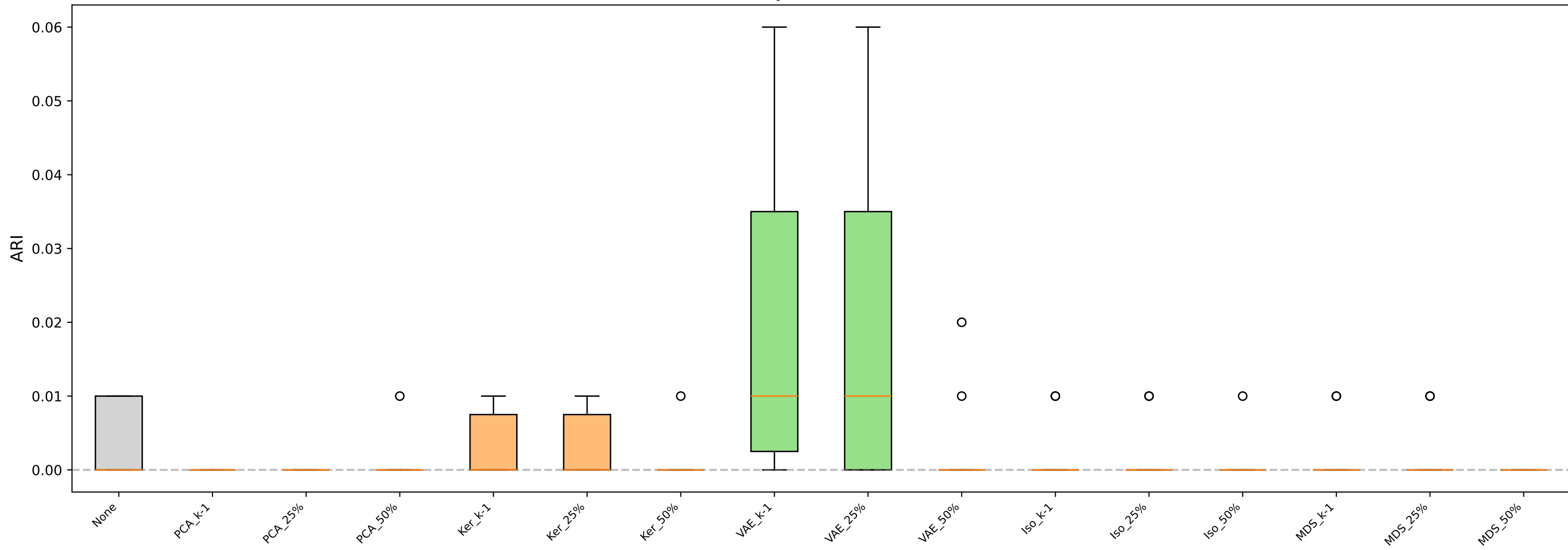
AHC - Synthetic (Circles)
