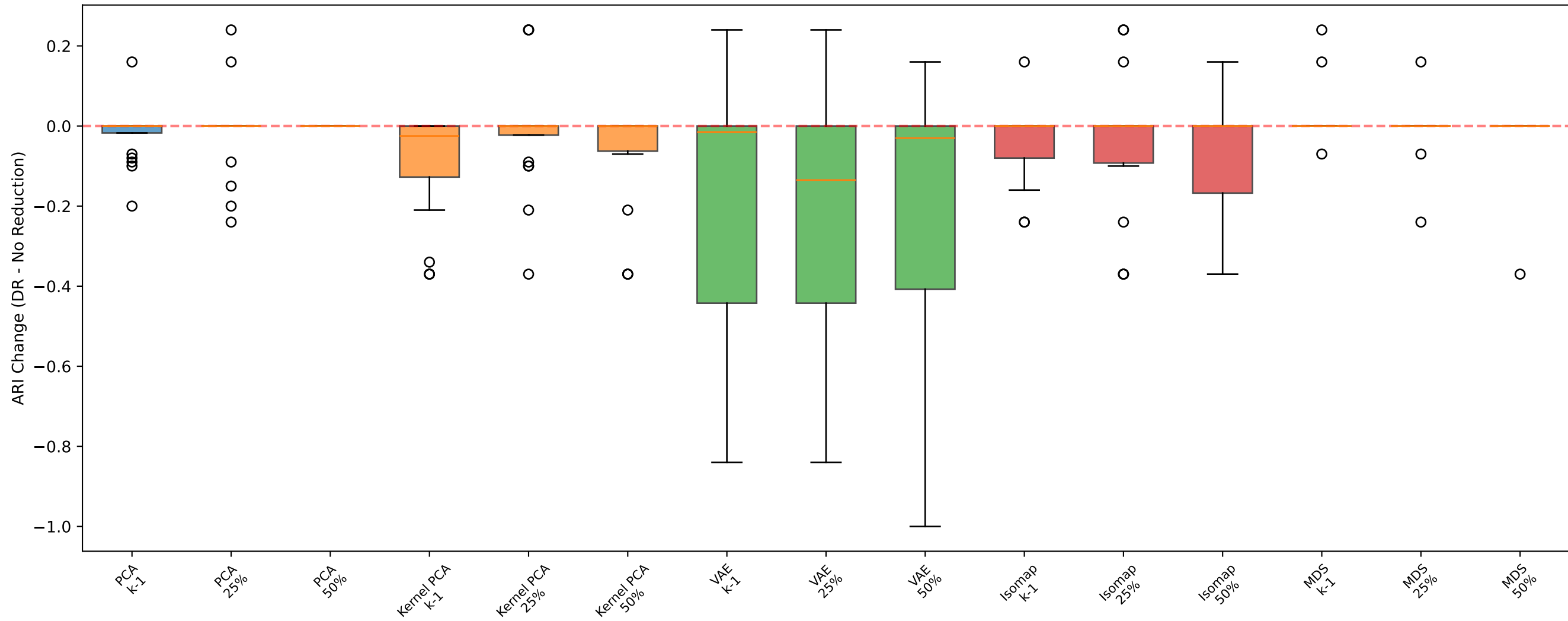
OPTICS - Repliclust: ARI Change by DR Method
