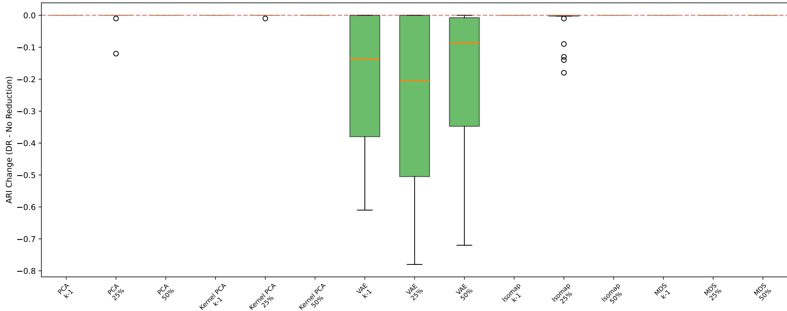
k-means - Repliclust: ARI Change by DR Method
