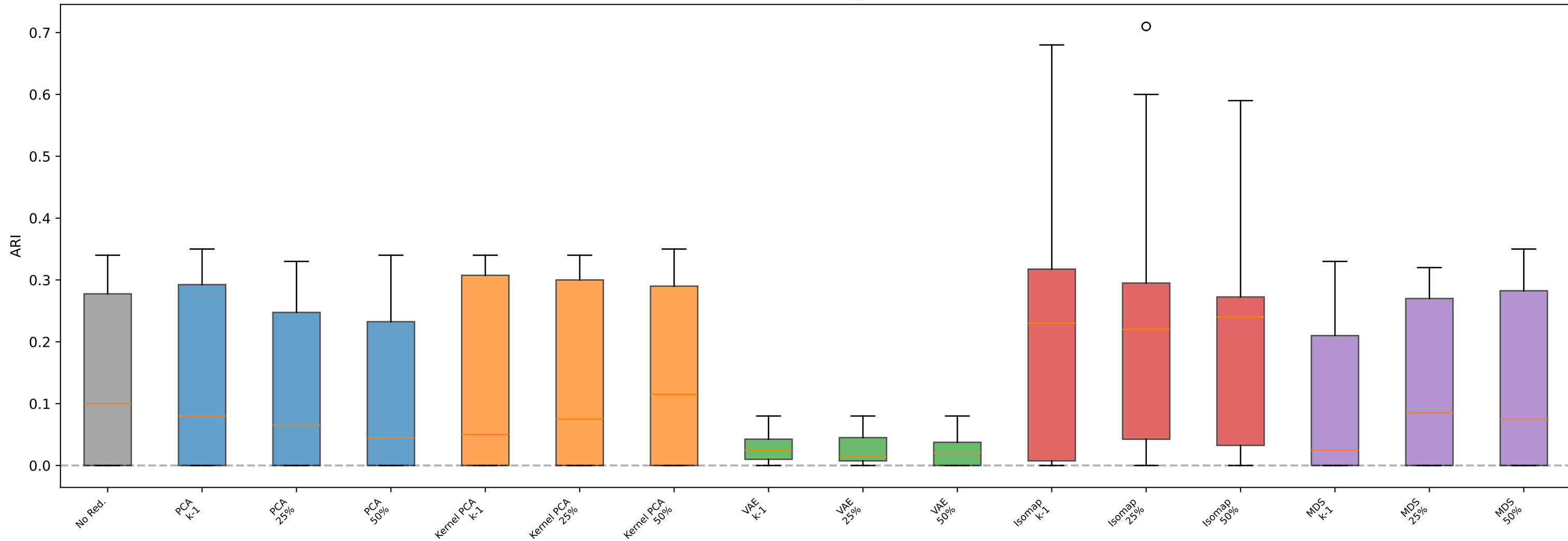
AHC — Synthetic_Circles
