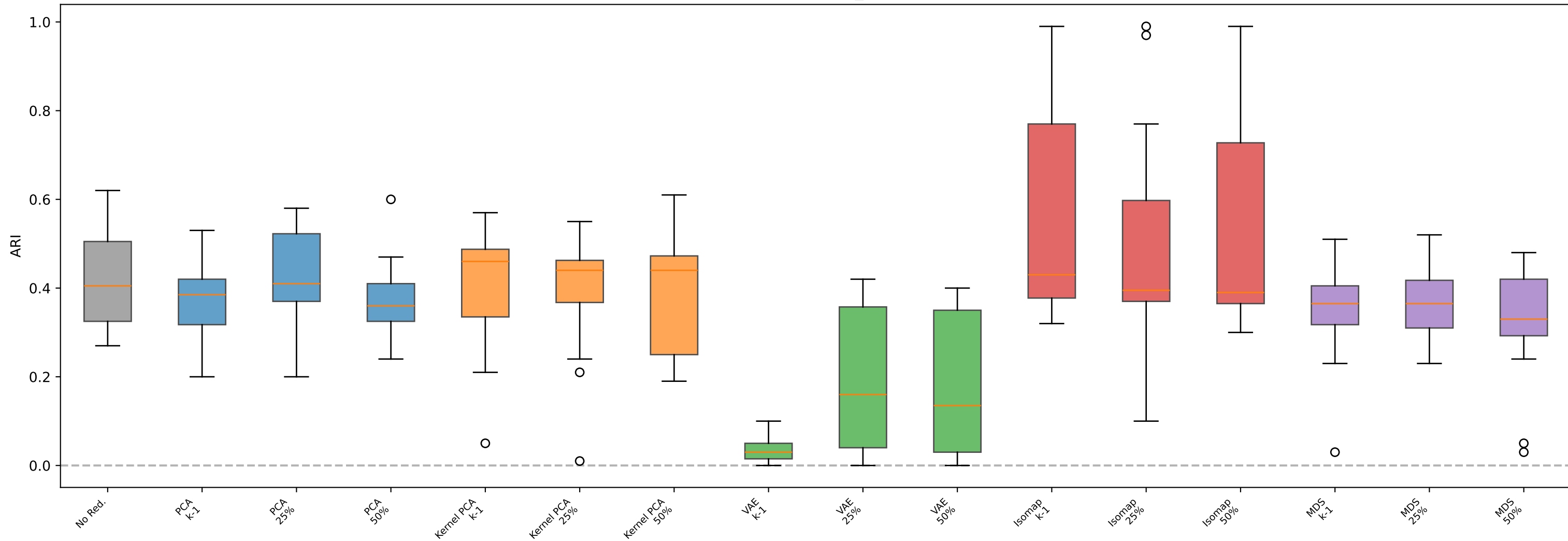
AHC — Synthetic_Moons
