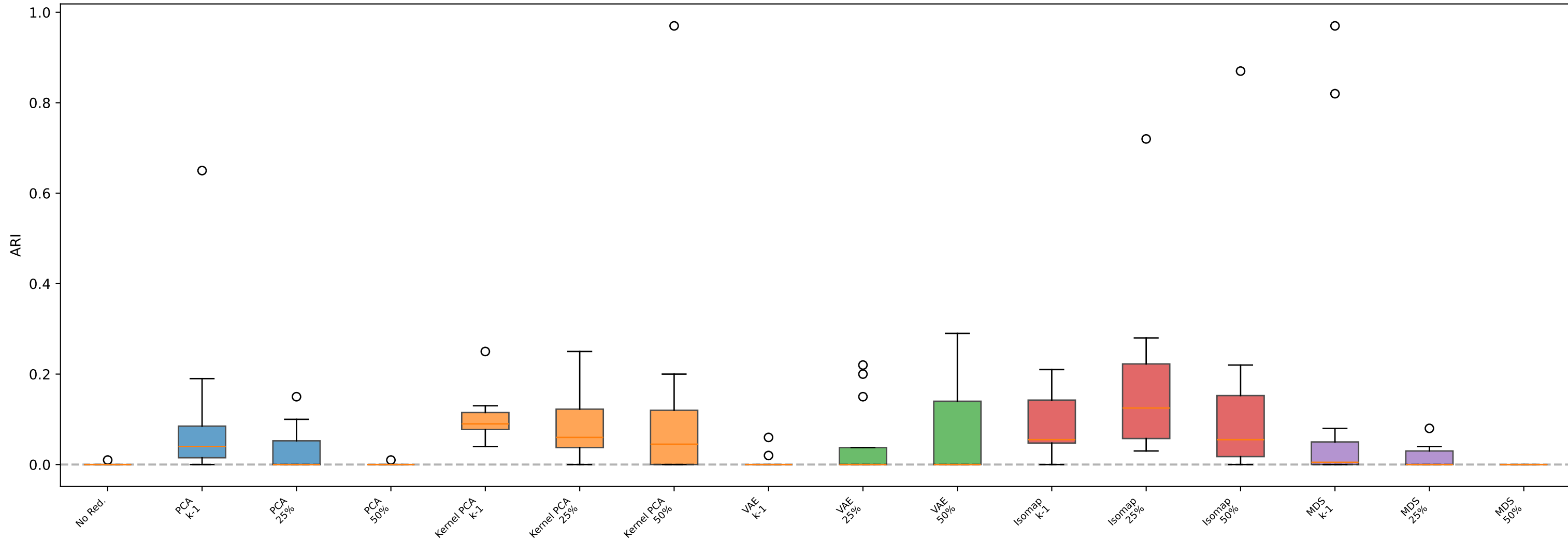
OPTICS — Synthetic_Moons
