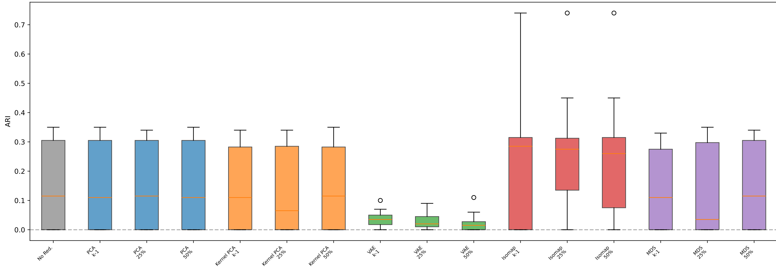
k-means — Synthetic_Circles
