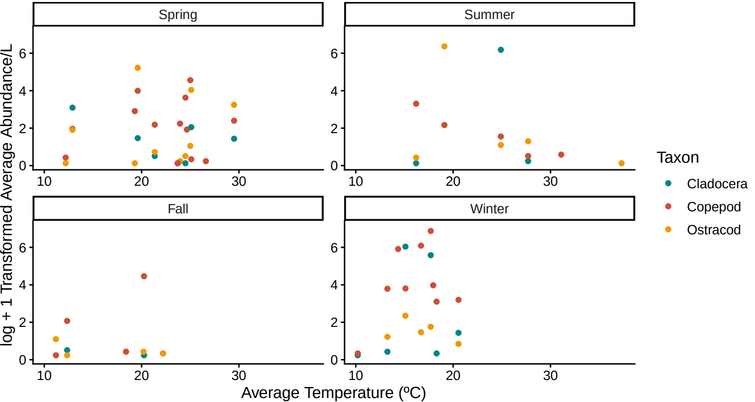
Average Abundance and Average Water Temperature by Season for Three Dominant Taxa
