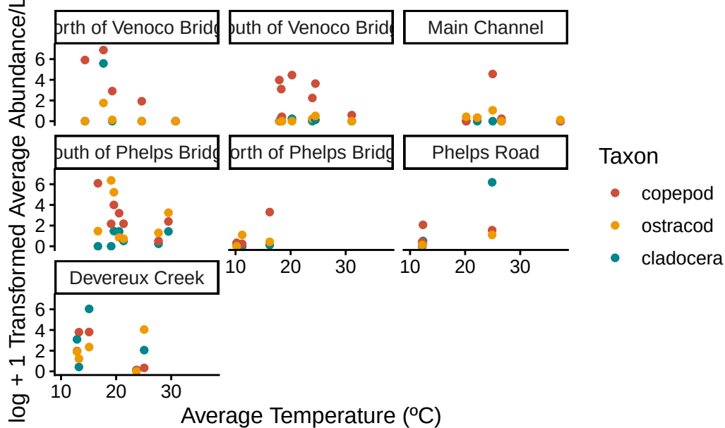
Figure 2 - Mean and Distribution of Invertebrate Abundance (log +1/L) for Three Tax
