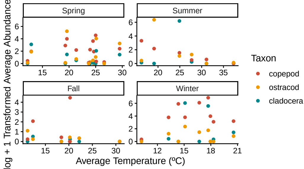
Seasonal Patterns Between Water Temperature and Log + 1 Abundance for Three Dominant Taxa
