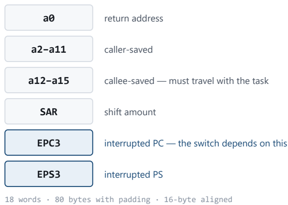
Figure 1. Saved-context frame. EPC3/EPS3 are what make a stack swap into an actual task switch.
