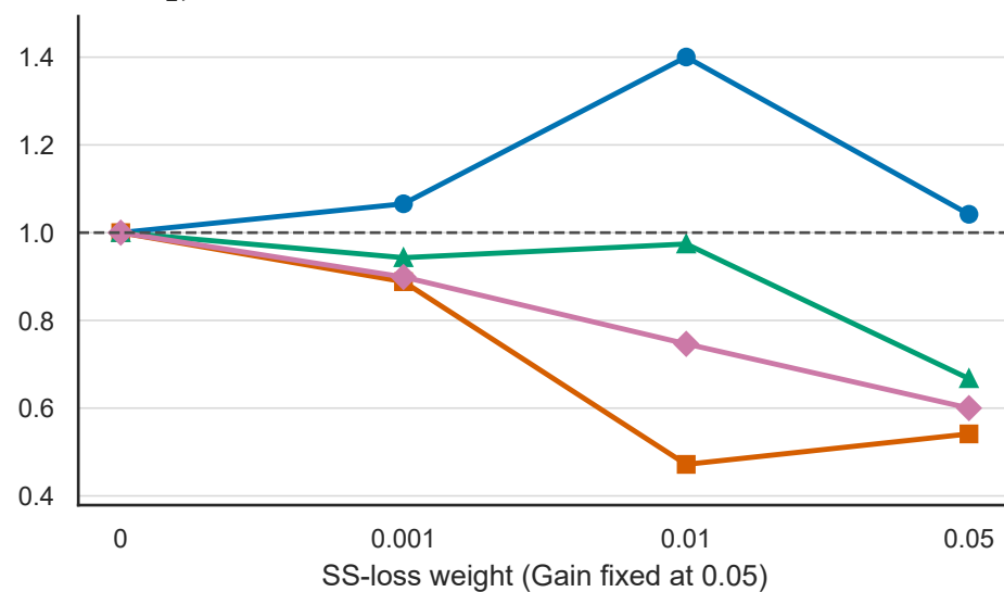
D SO 2 , Horizon 18
