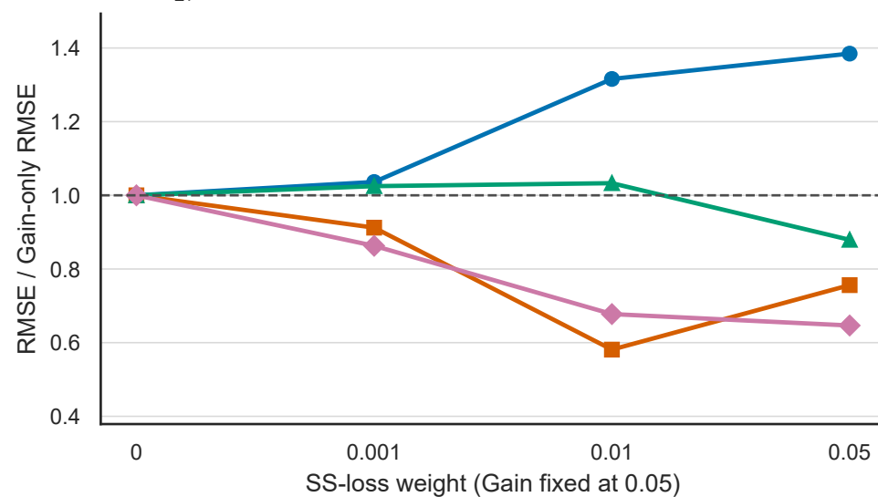
C SO 2 , Horizon 1
